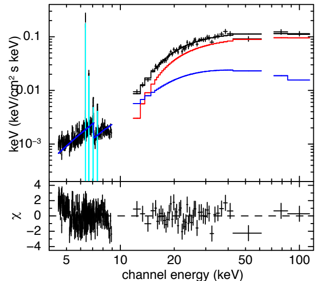
Fig. 5. (Top) The broad band (4.5–120 keV) \nu F\nu spectrum of NGC 4945, on which BC model is superposed. The data are shown in black points and the models in colored lines; the absorbed intrinsic power-law in red, the cold reflection component in blue, and emission lines in cyan. (Bottom) The residuals from this fit.
